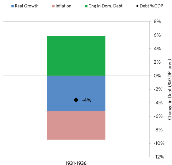
Deleveraging Attribution: Reflation Period
